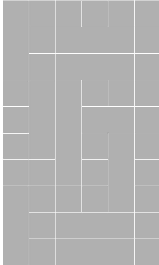
Scheme 4
