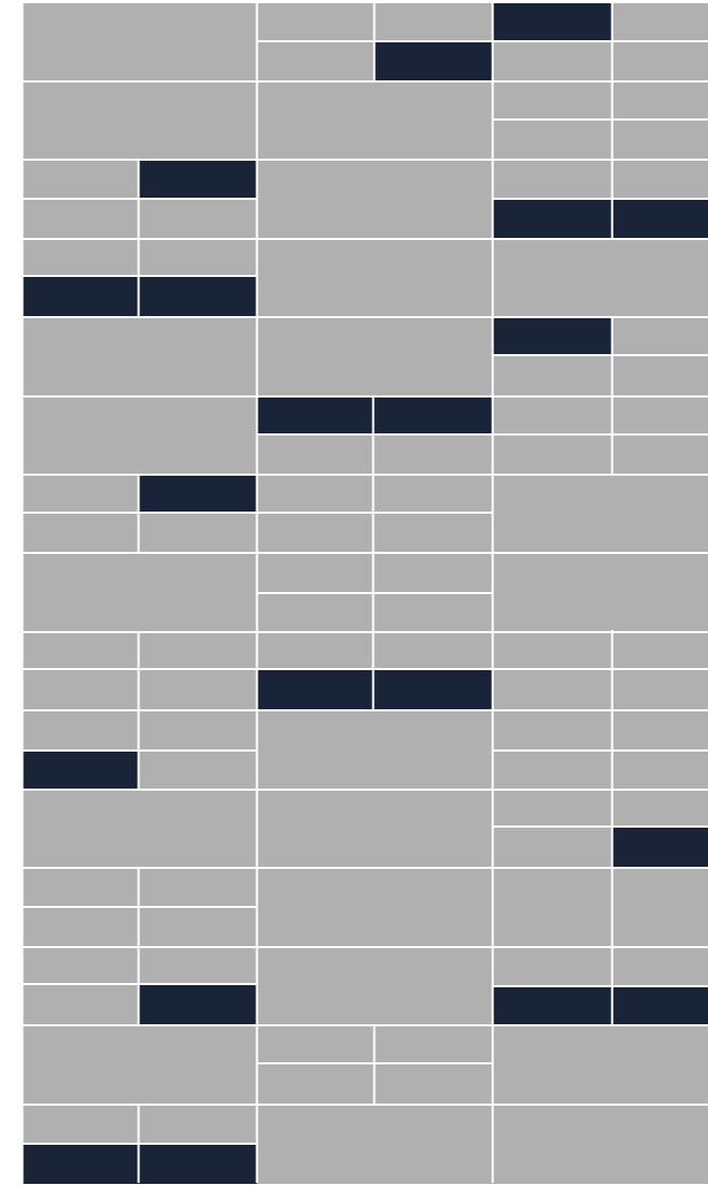
Scheme 6
