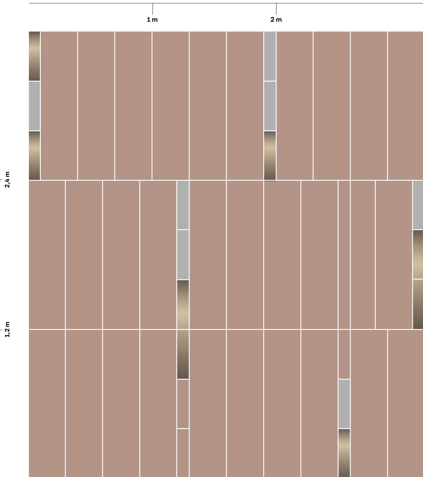
Scheme 1
