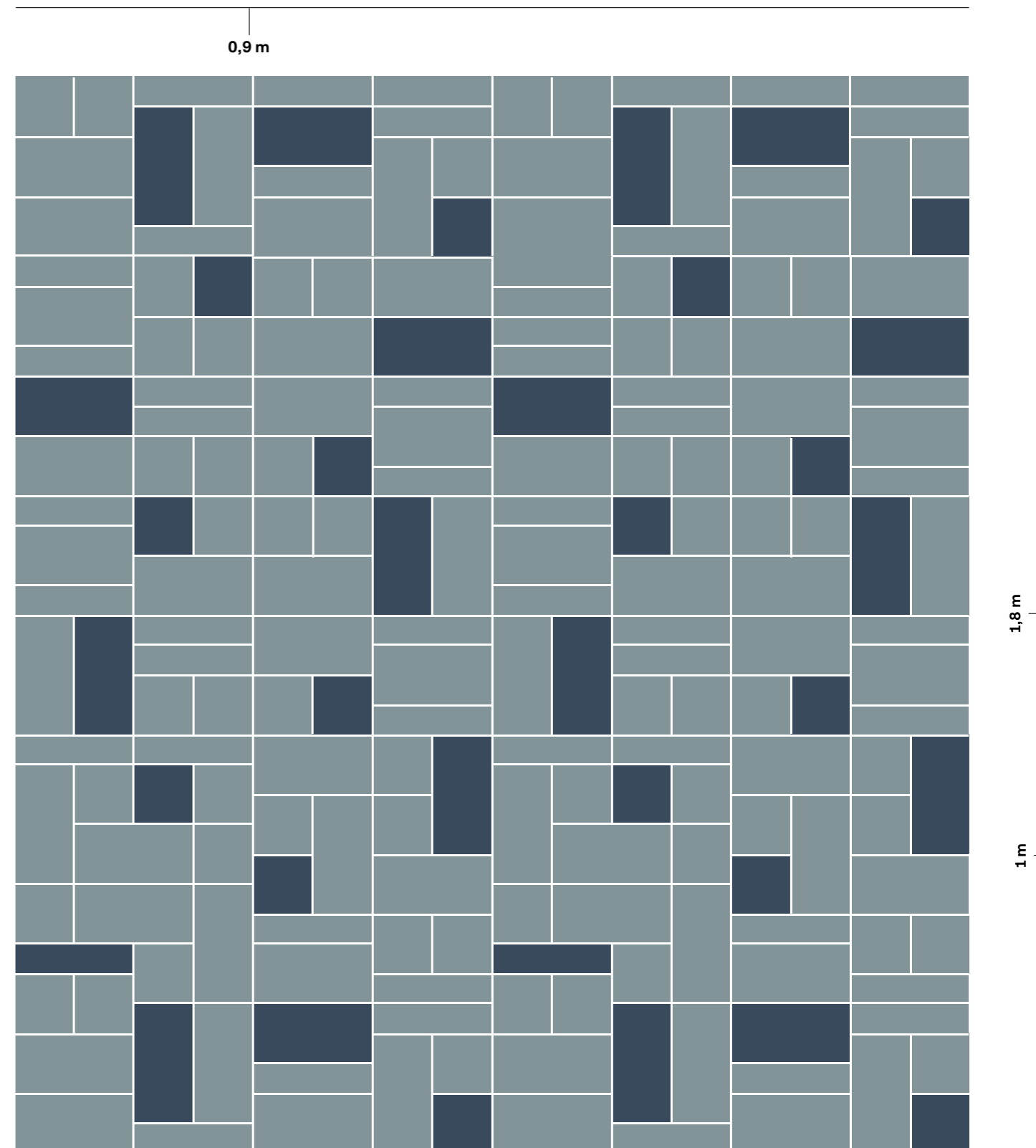
Scheme 2
